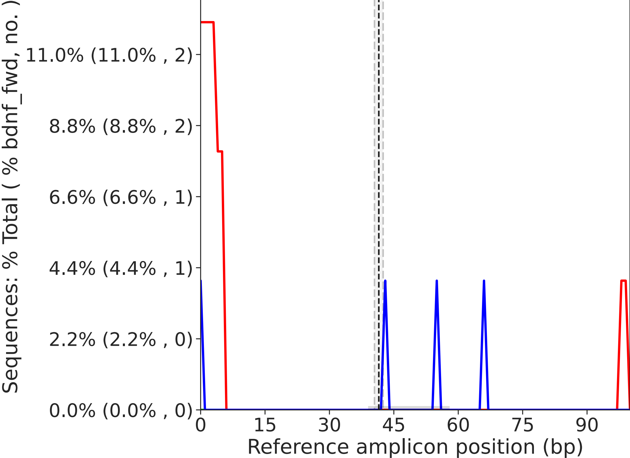
Mutation position distribution: bdnf_fwd
