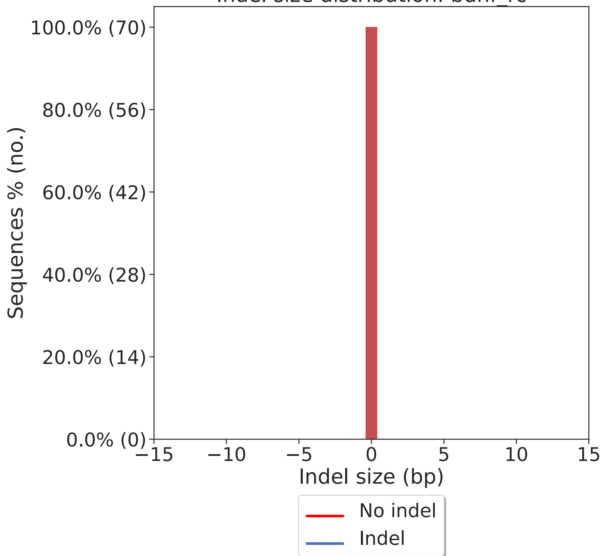
Indel size distribution: bdnf_rc
