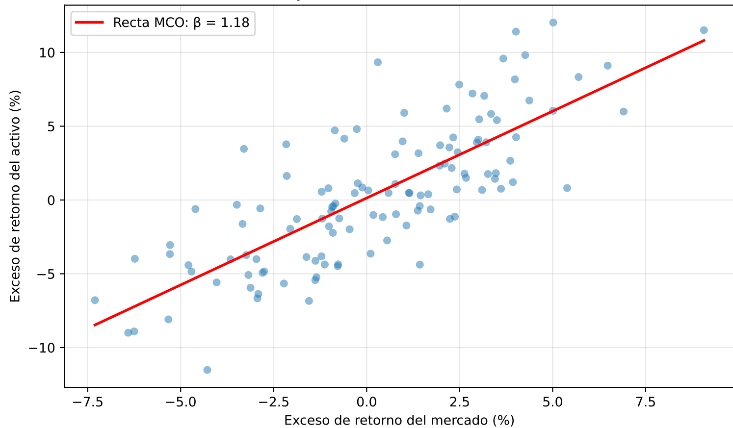
Security Characteristic Line — R^2 = 0.60
