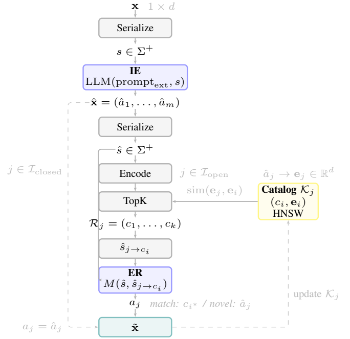
Fig. 1. Vehicle normalization pipeline. The raw record \mathbf{x} is serialized and passed to the LLM for attribute extraction (IE). Closed-domain attributes (dashed bypass) are assigned directly. Open-domain attributes are embedded, matched against a knowledge catalog \mathcal{K}_j via HNSW, and resolved (ER) by comparing serialized vehicle descriptions. Novel entities expand the catalog.
