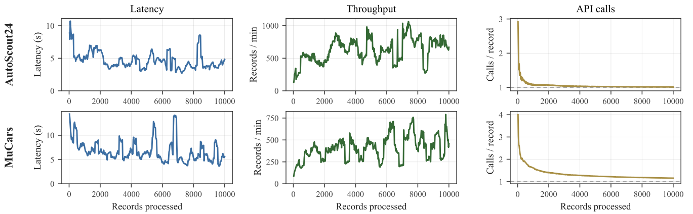
Fig. 5. Computational efficiency over a 10,000-record stream. Left: latency; center: throughput; right: API calls per record (dashed: extraction floor).
