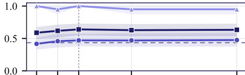
Novelty detection
