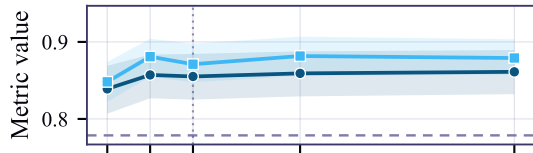
Model normalization
