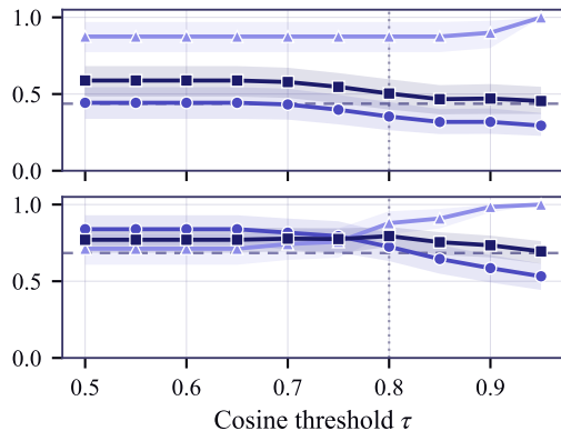
Novelty detection
