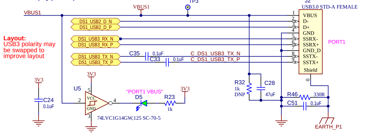
USB3.1(Type-A) Downstream Port 1
