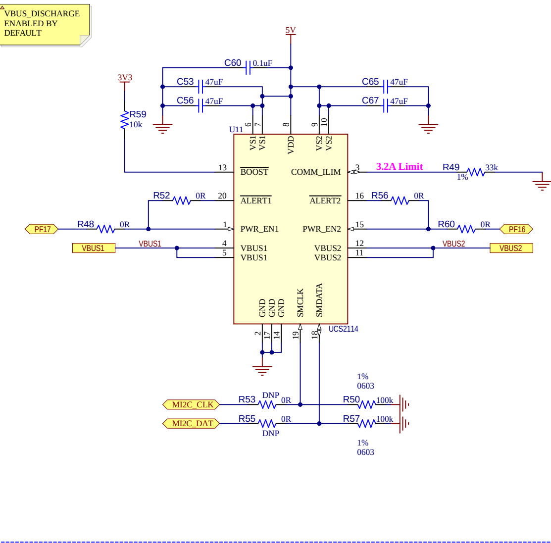
UCS2114 Power Switch For Port1 and Port2
