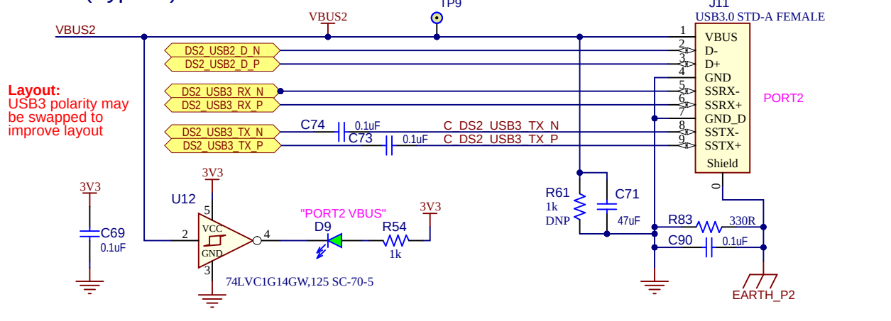
USB3.1(Type-A) Downstream Port 2
