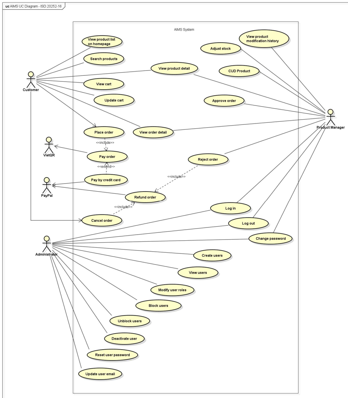
Figure 1. AIMS Use Case Diagram
