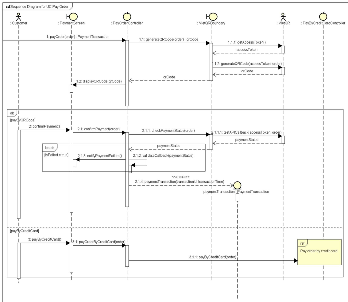
Figure 6. UC Pay Order Sequence Diagram
