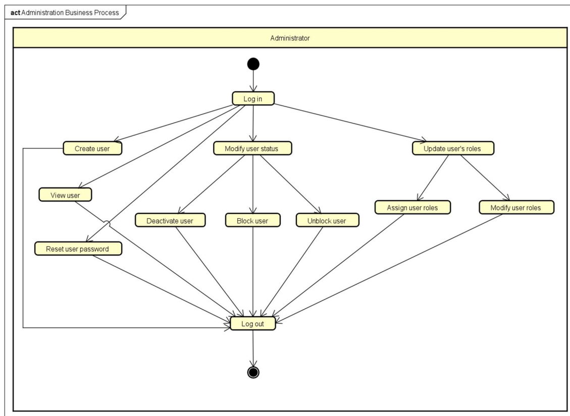
Figure 4. AIMS Administration Process
