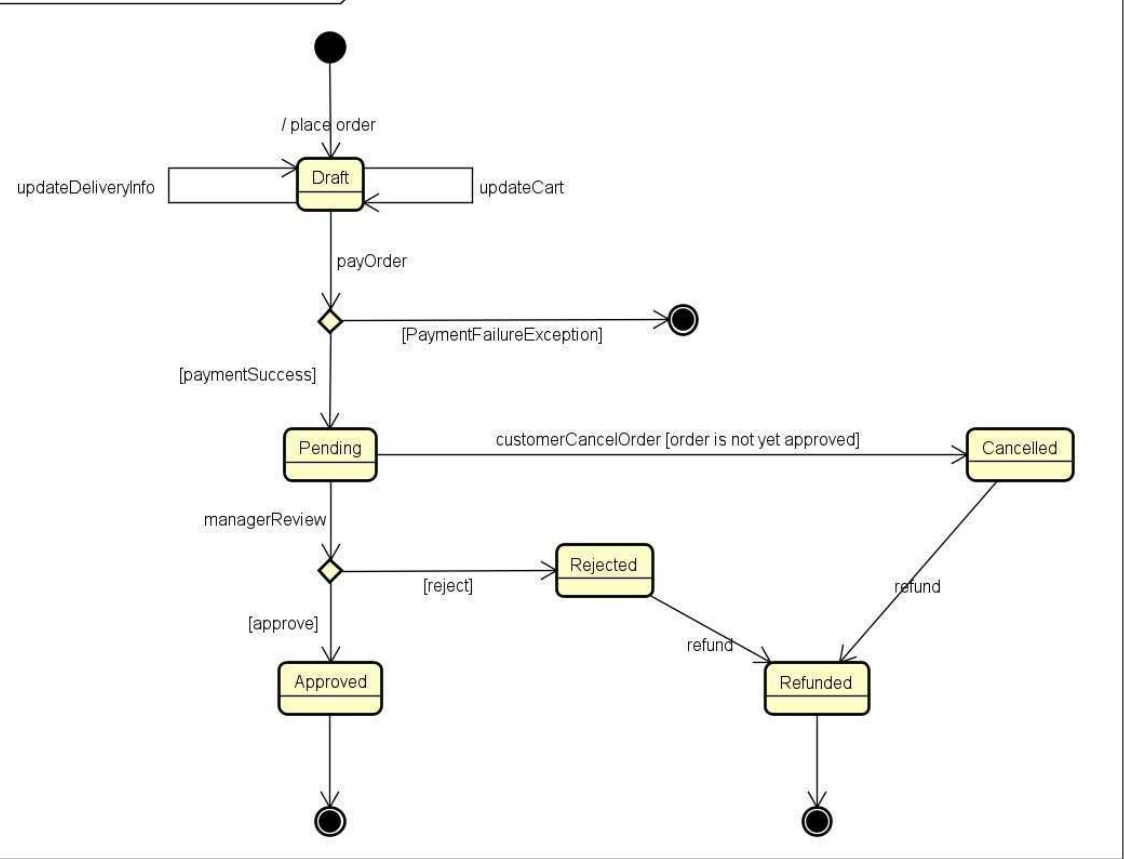
stm State machine Diagram for Entity Order
