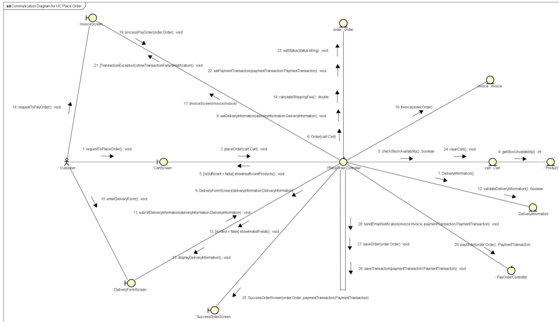
Figure 7. UC Place Order Communication Diagram
