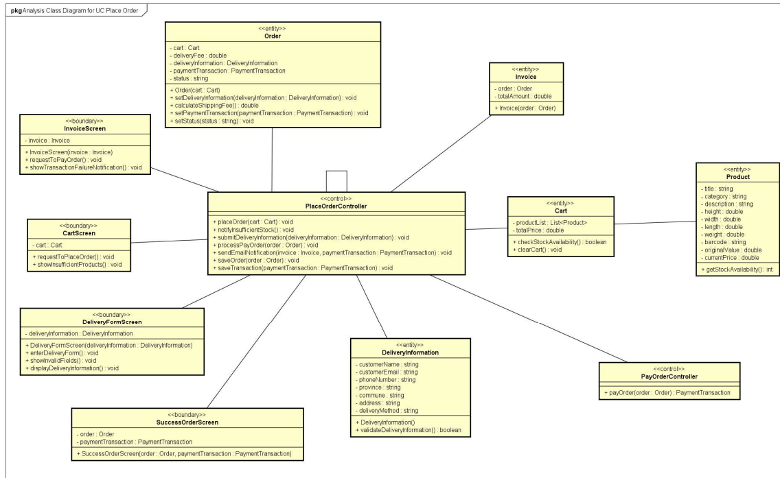
Figure 9. UC Place Order Analysis Class Diagram
