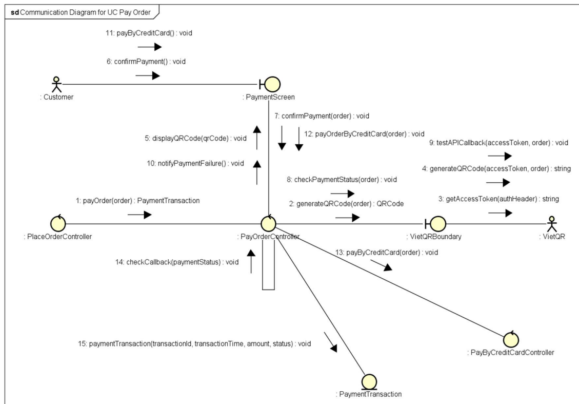
Figure 8. UC Pay Order Communication Diagram
