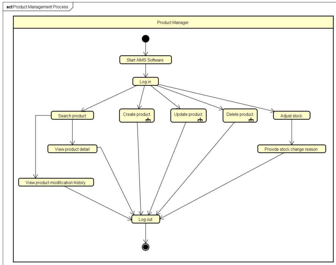
Figure 3. AIMS Product Management Process
