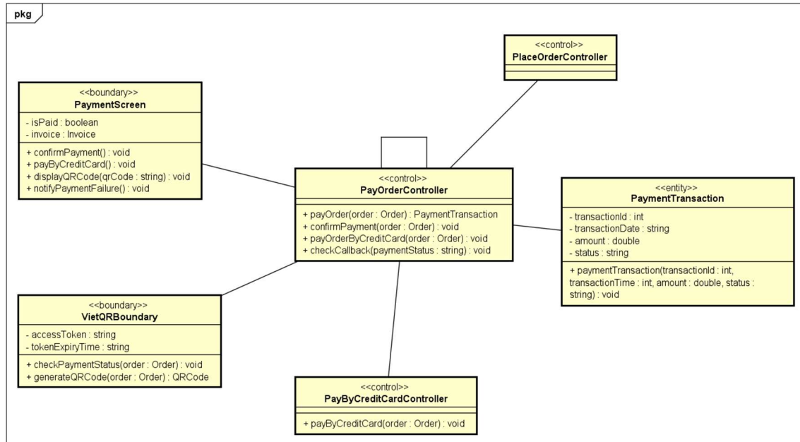
Figure 10. UC Pay Order Analysis Class Diagram
