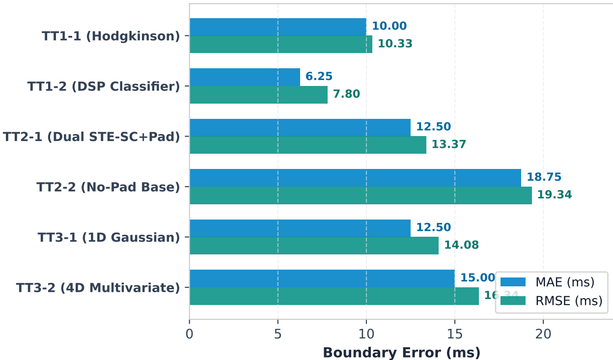
Overall VAD Boundary Error Benchmark (4 Test Recordings)
