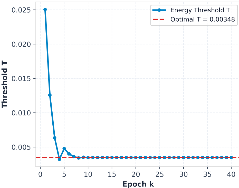
TT1 Intermediate Training: 40-Epoch Bisection Convergence on Training Set Search Interval Halving (Domain [10^{-4}, 0.05] )
