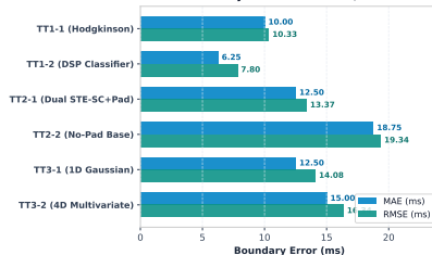
Overall VAD Boundary Error Benchmark (4 Test Recordings)
