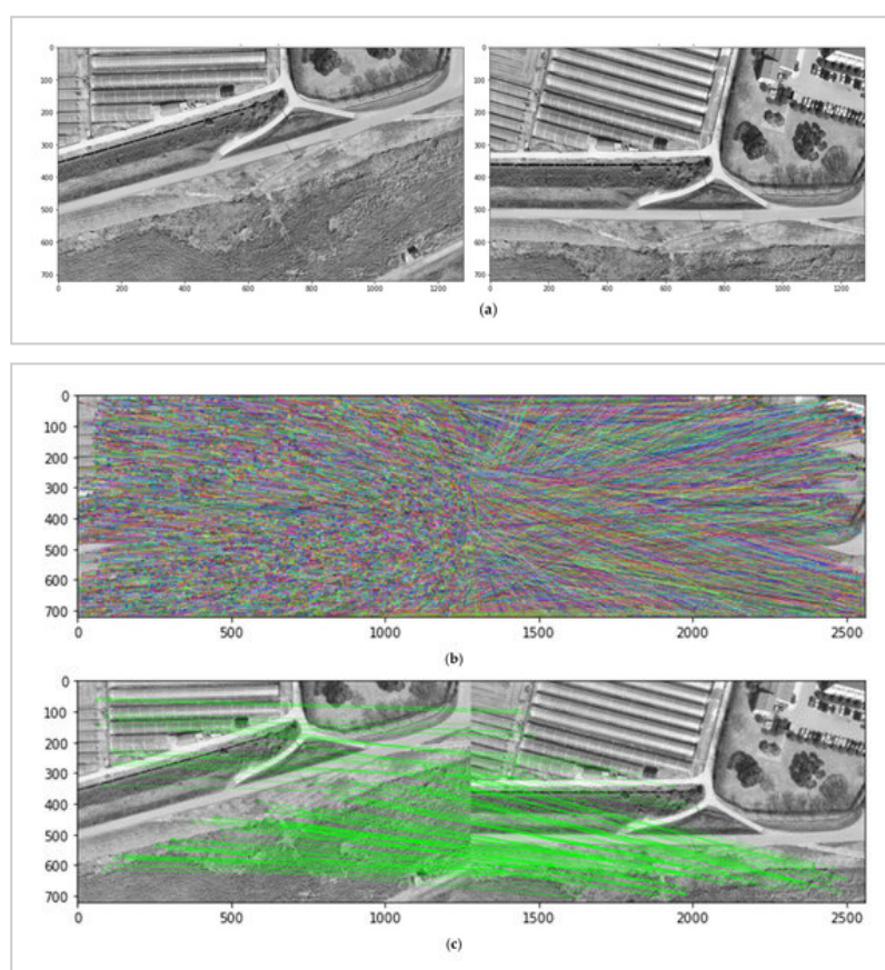
Figure 9. Results of applying the random sample consensus (RANSAC) algorithm: (a) Gray-scale images; (b) before RANSAC application; (c) after RANSAC application.
