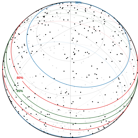
Long-period comets (n = 610)
