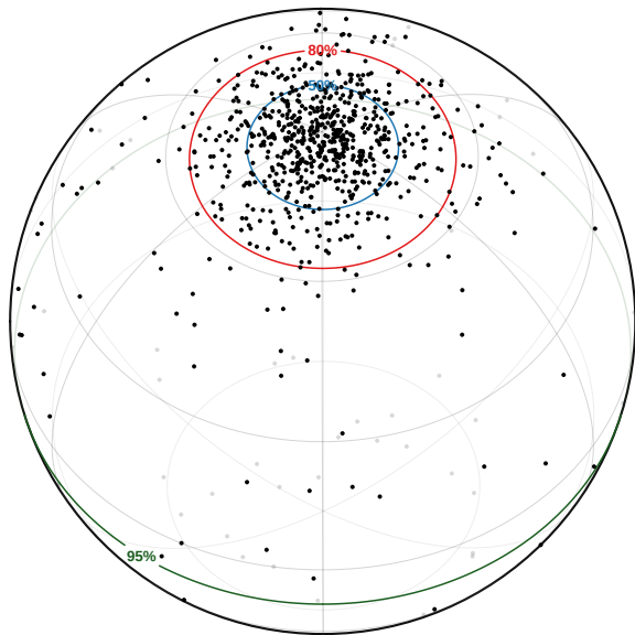
Short-period comets (n = 784)
