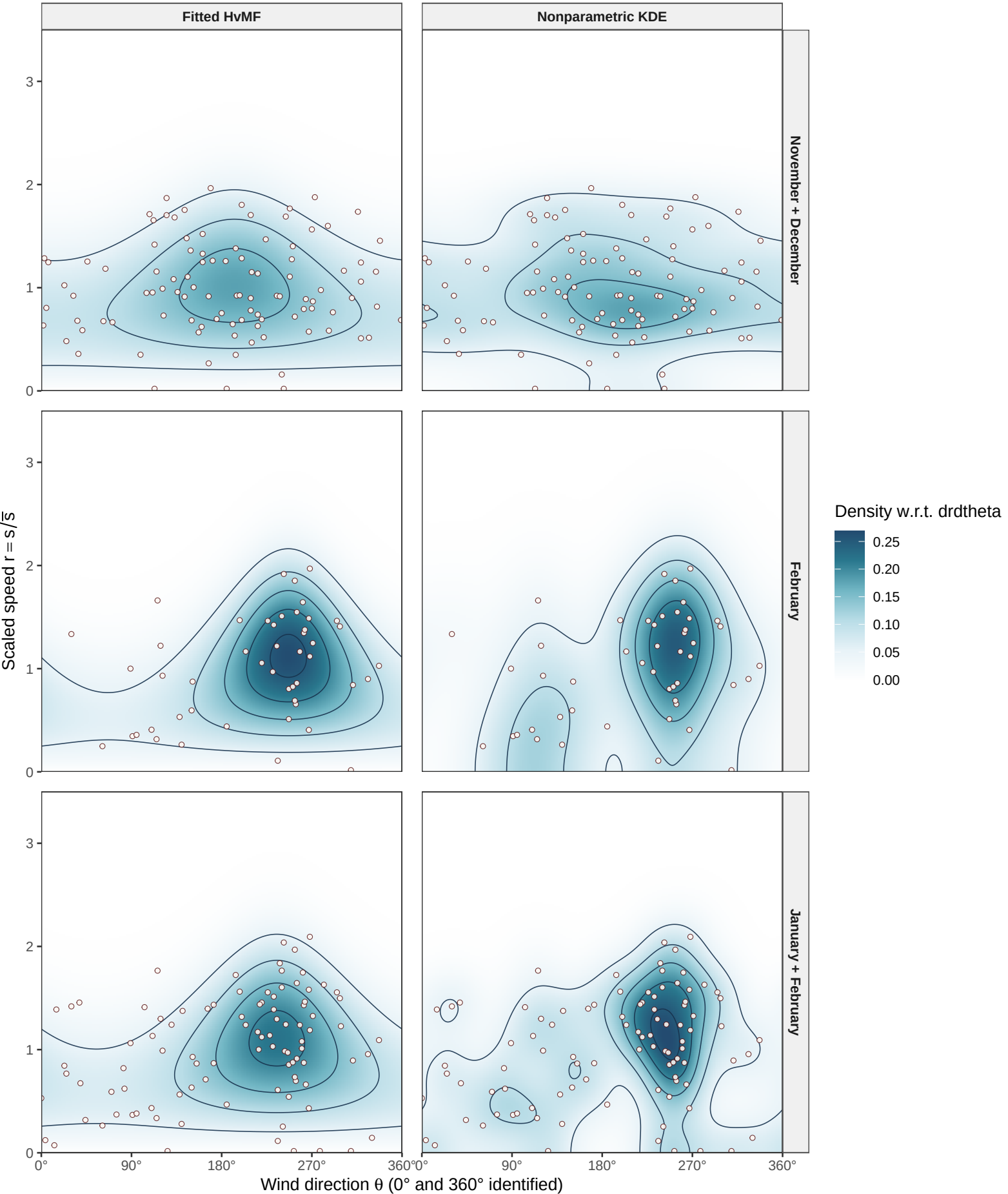
Risø 125 m wind data on the unwrapped cylinder start4: days 4, 8, 12, 16, 20, 24, 28; closest-to-noon observations, 1996–2003
