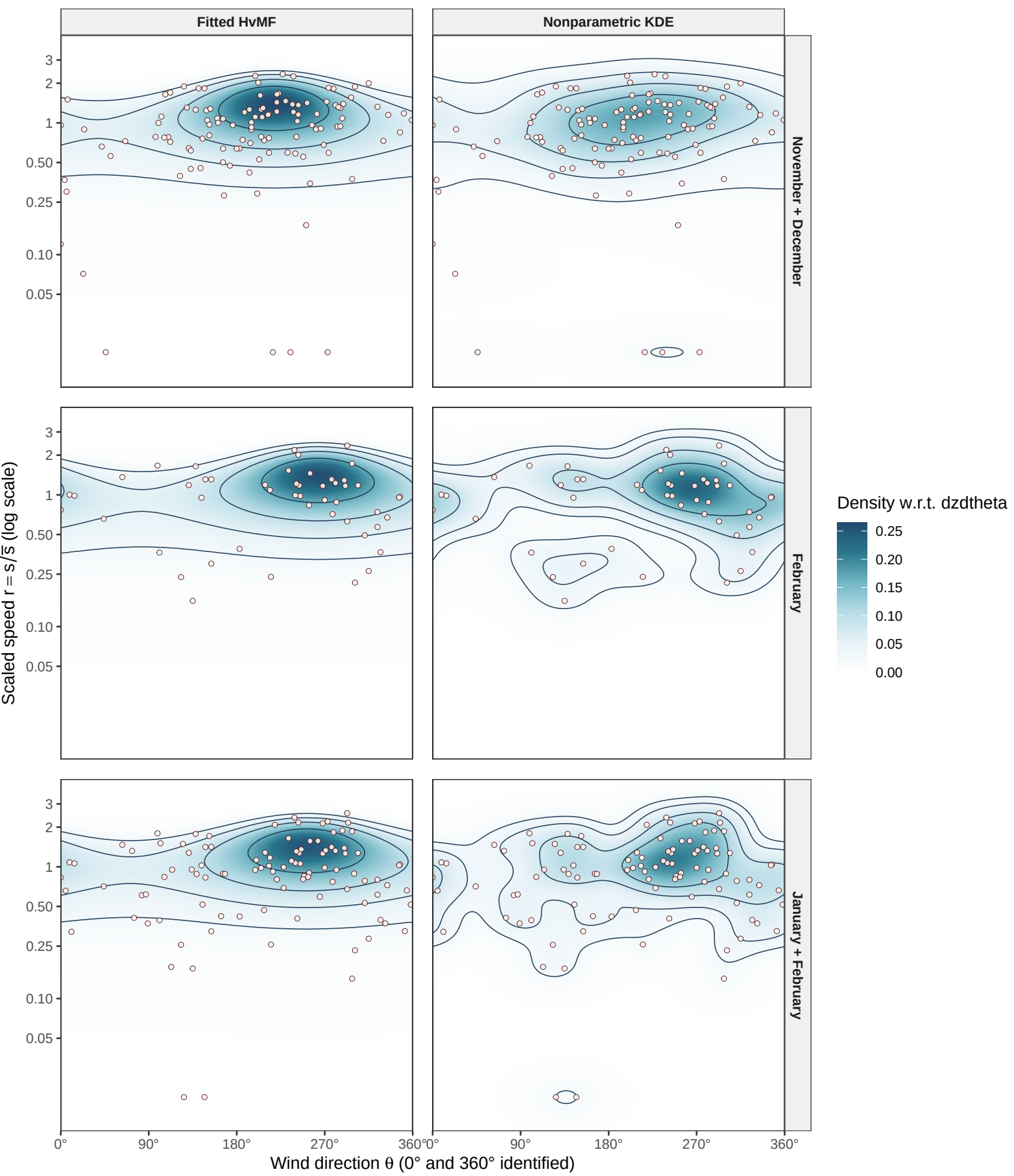
Risø 125 m wind data on the unwrapped log-speed cylinder start1: days 1, 5, 9, 13, 17, 21, 25, 29; closest-to-noon observations, 1996–2003; HDR contours: 25%, 50%, 75%, 90%
