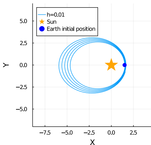
Euler's method (position)
