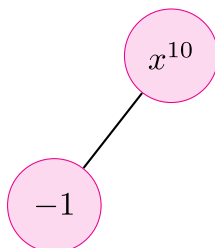
Figure 6: Sparse representation of x^{10} - 1
