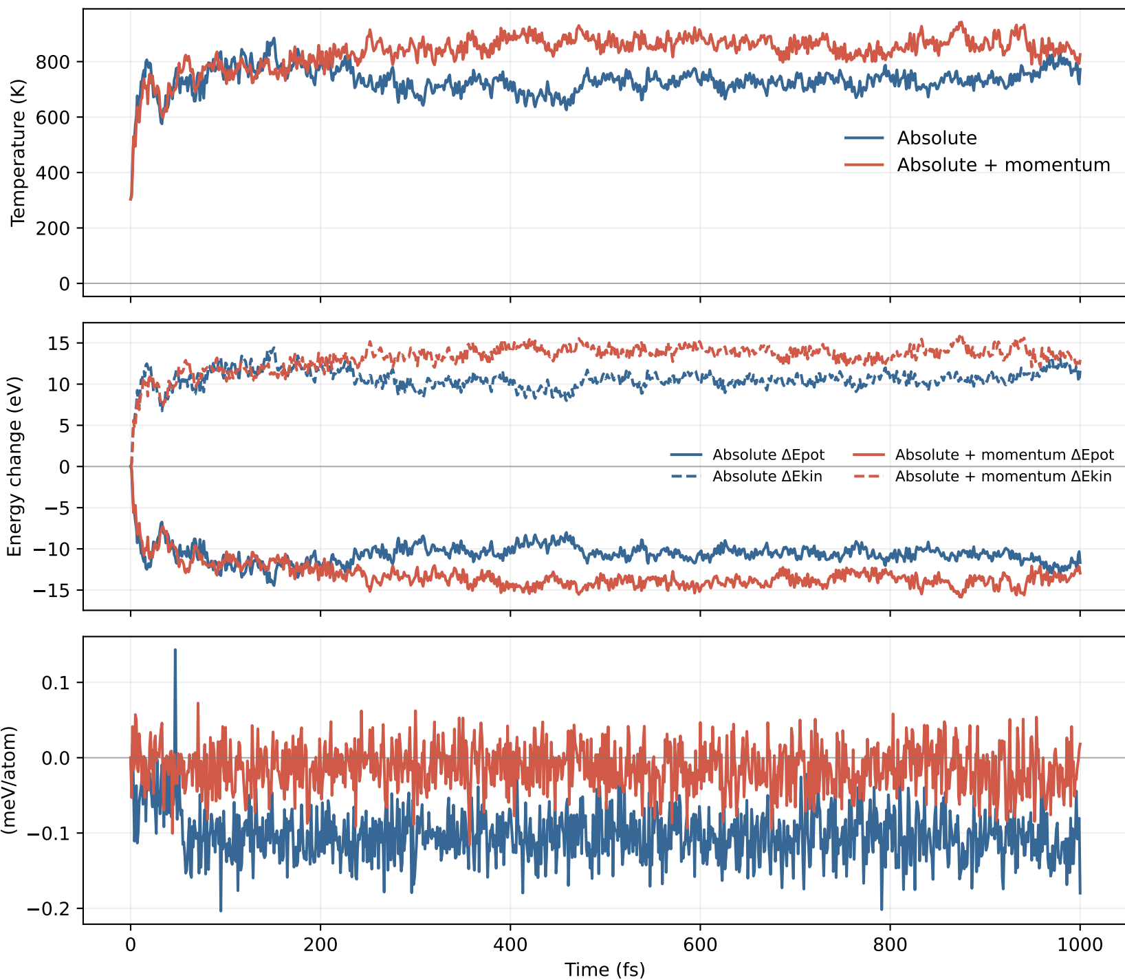
Representative matched rollout selected by median pair temperature train seed 2; axis=velocity; velocity seed=0; config=0
