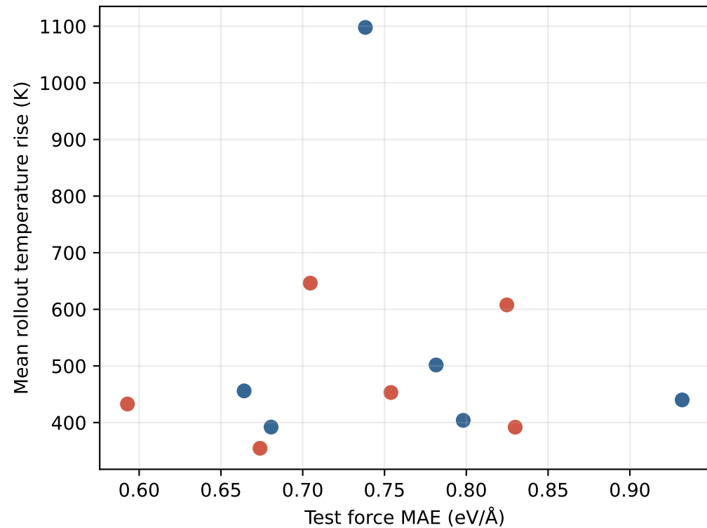
Static test metrics versus dynamical heating
