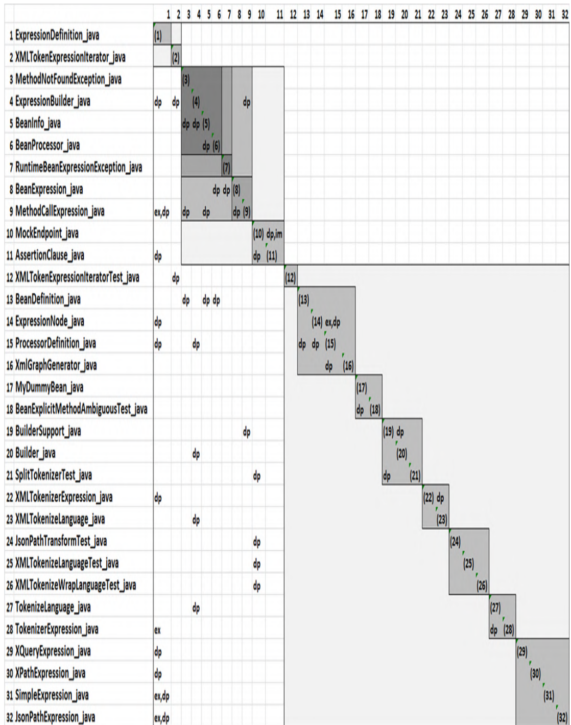
Figure 23.1 A DSM of Apache Camel showing structural dependencies
