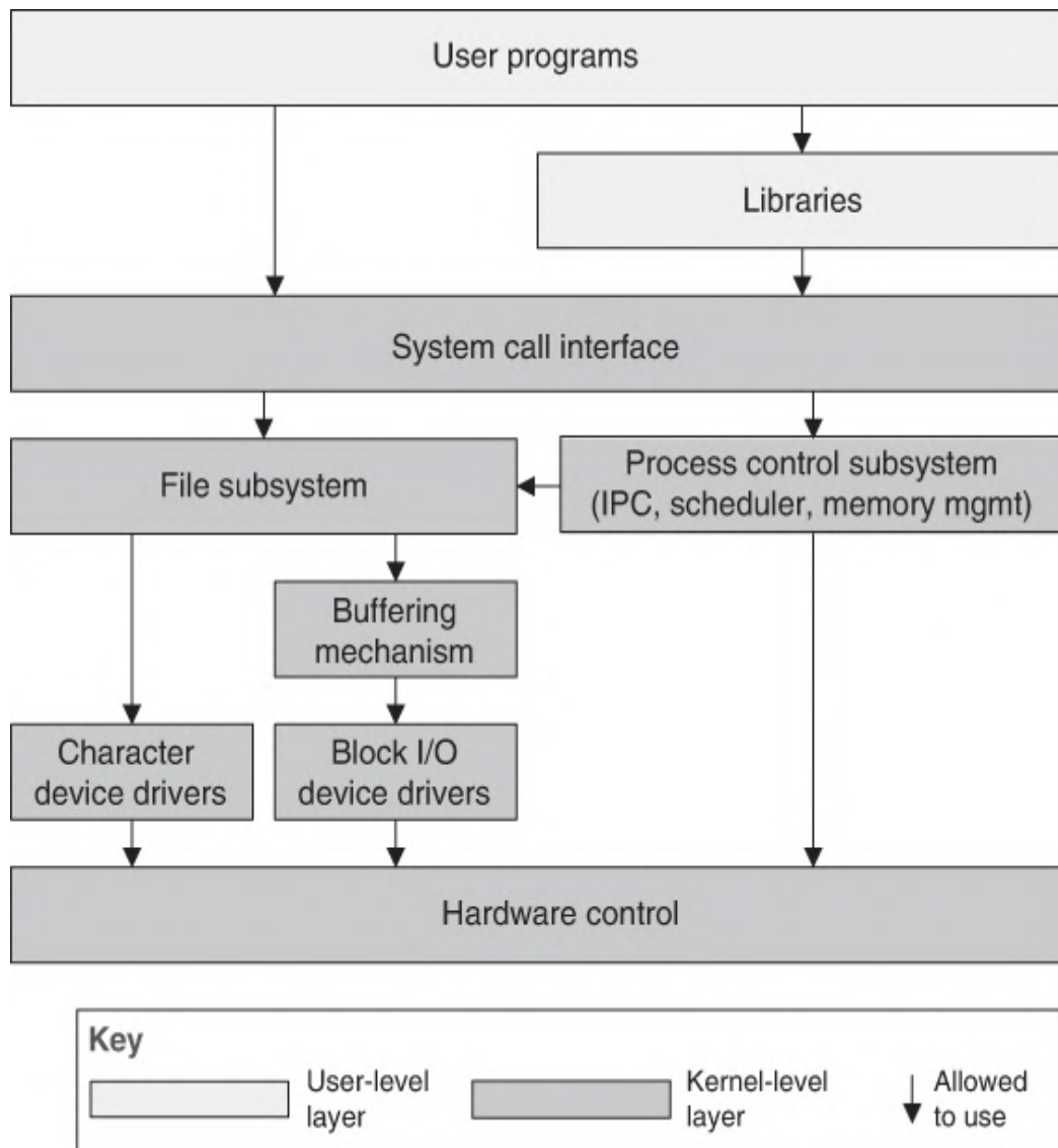
Figure 1.7 Layer structure
