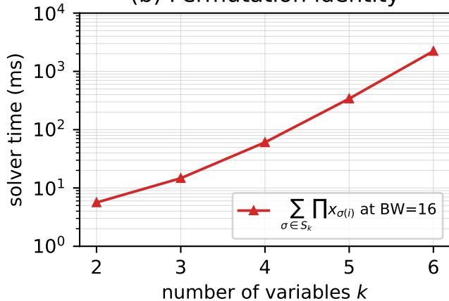
(b) Permutation identity
