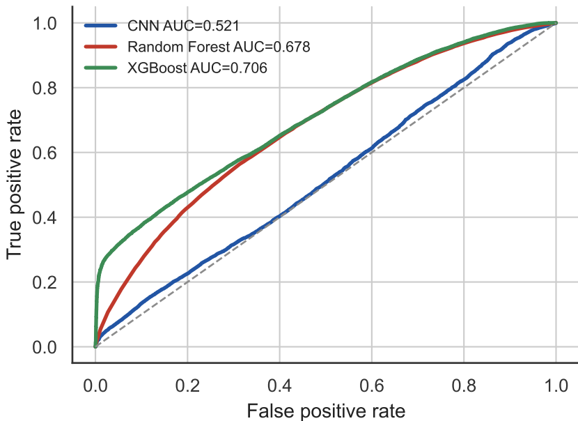
Run-holdout pooled ROC
