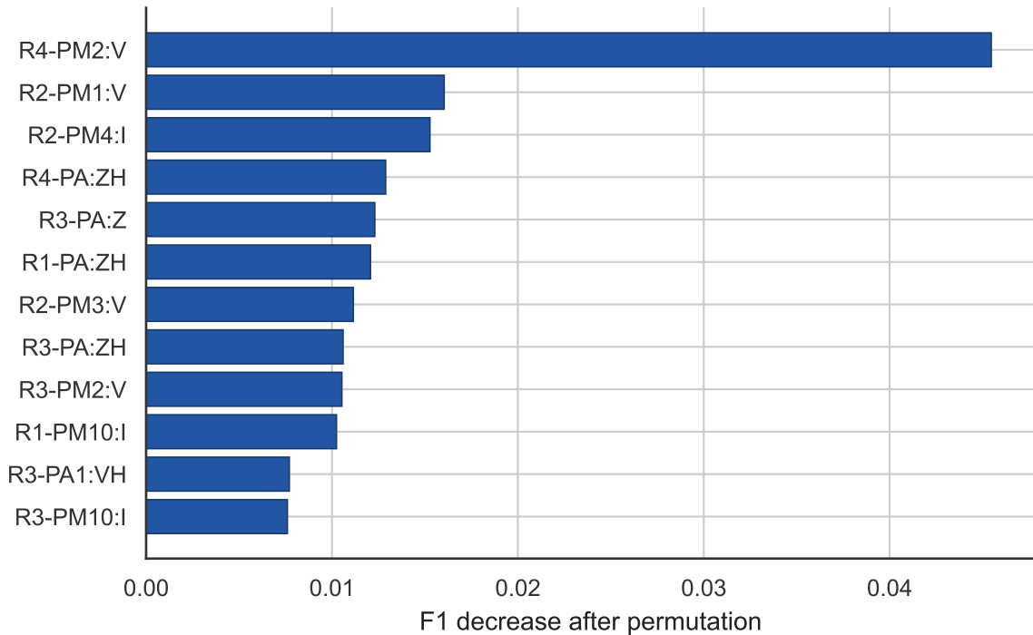
Top held-out feature importance
