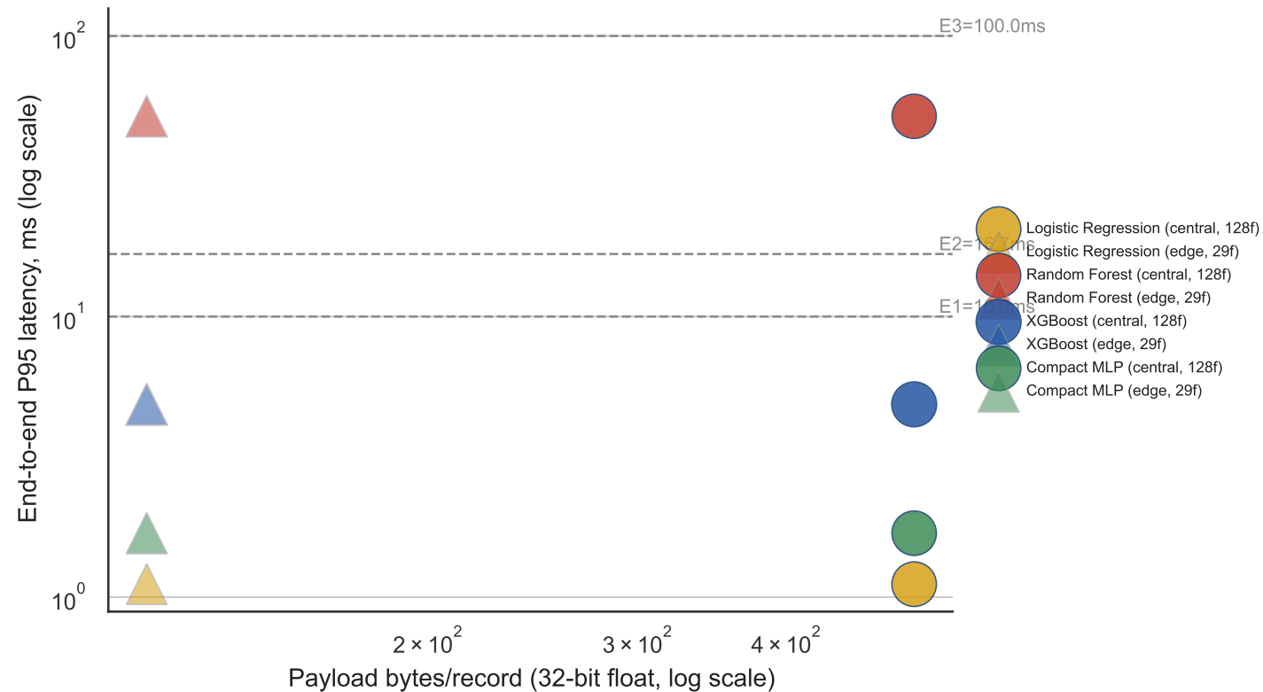
Trade-space: payload, latency, and run-aware ROC-AUC (marker size)
