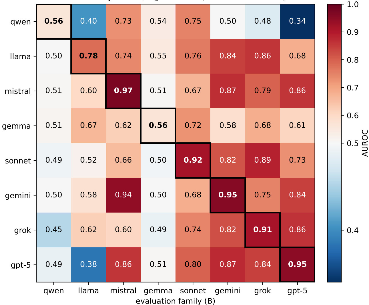
Cross-family AUROC, eight families (four frontier vendors)
