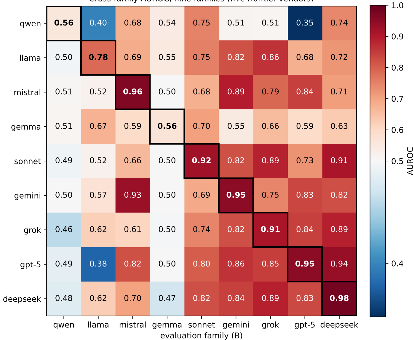
Cross-family AUROC, nine families (five frontier vendors)
