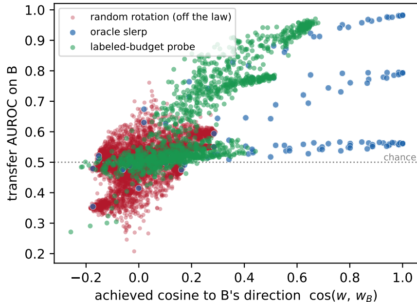
B. One law: AUROC is governed by the achieved cosine, however the rotation is produced
