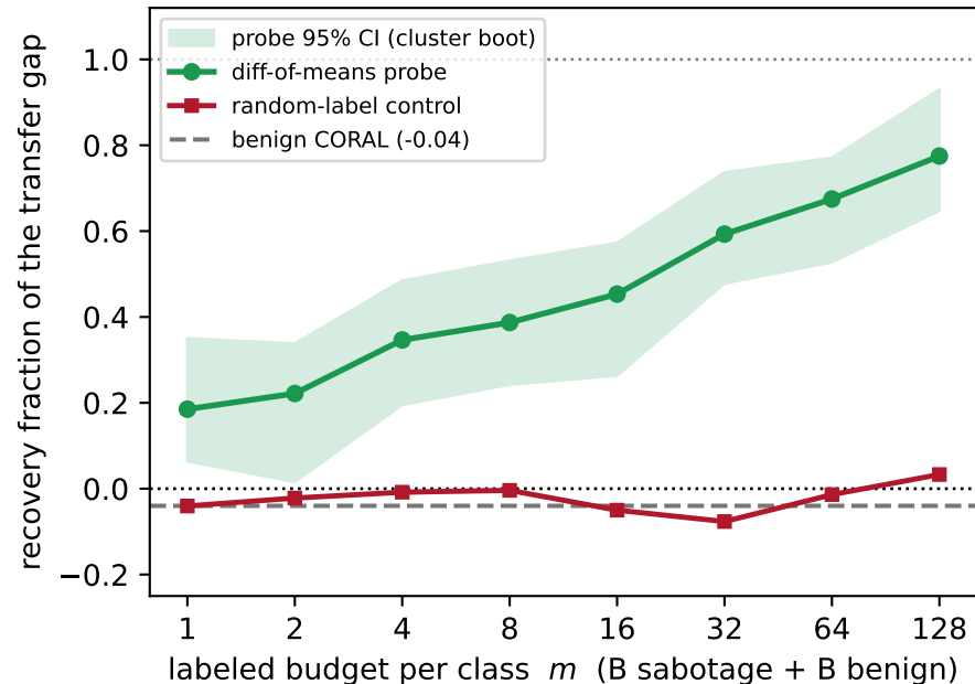
C. Labeled-budget recovery curve (a small labeled set rotates A most of the way)
