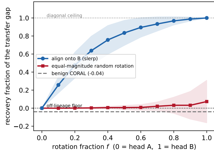
A. Rotate the head onto B \rightarrow AUROC recovers (random rotation of equal angle does not)
