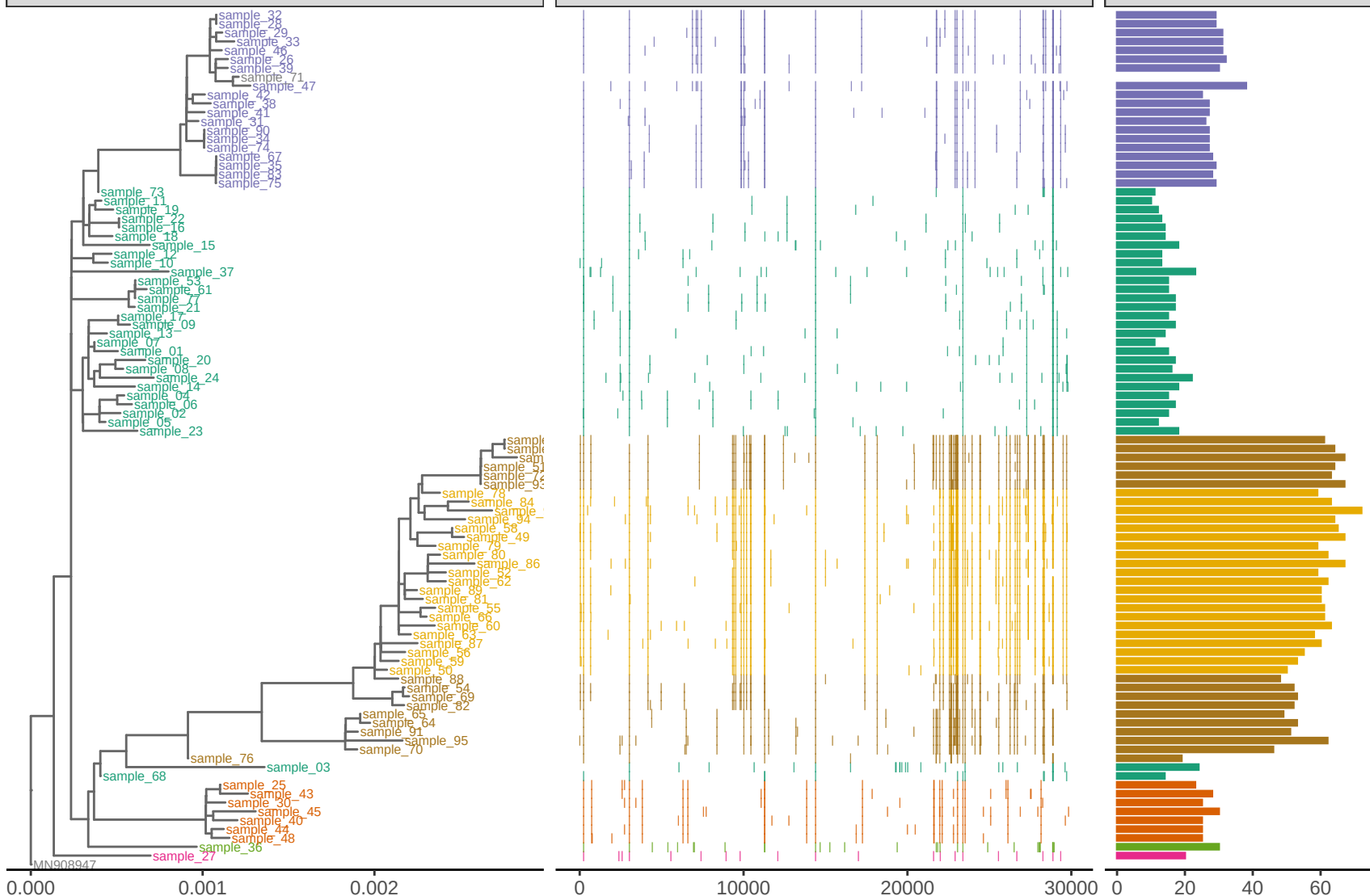
Tree
