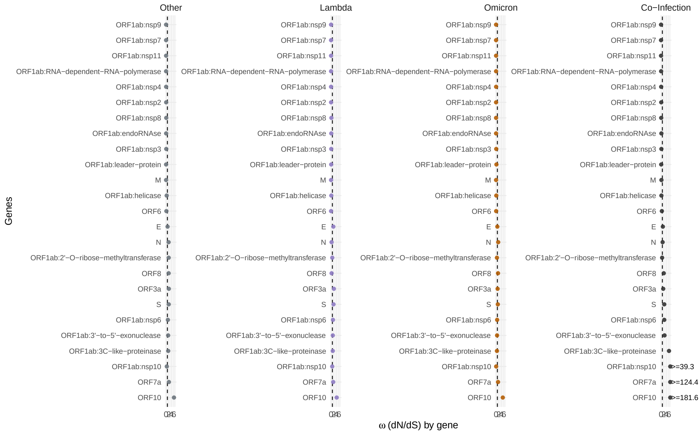
Gene-level dN/dS
