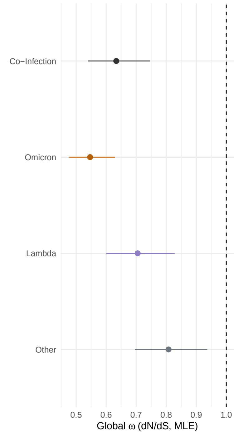
Global dN/dS
