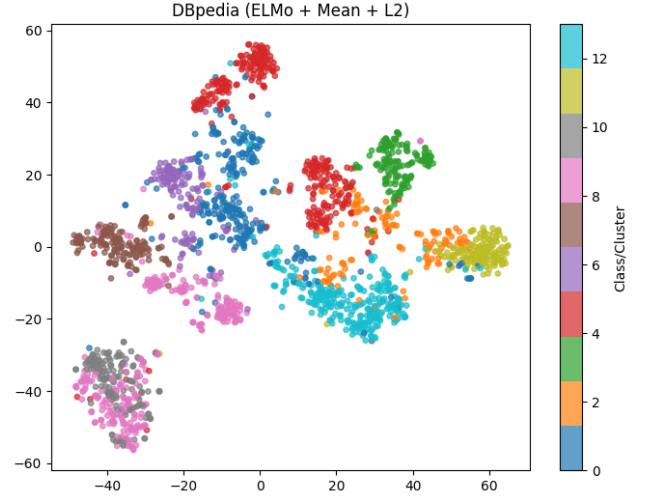
Figure 18: t-SNE visualization of ELMo embeddings with mean pooling and \ell_2 normalization on DBpedia.
