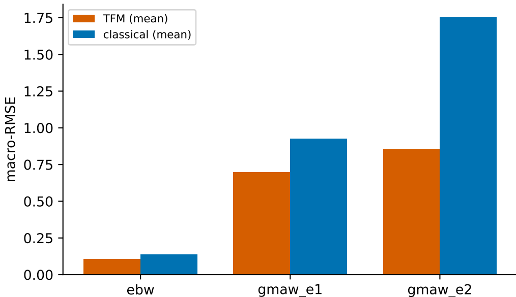
External validity across datasets
