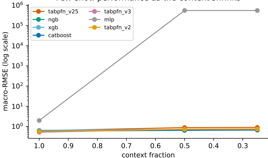
Few-shot: performance as the context shrinks
