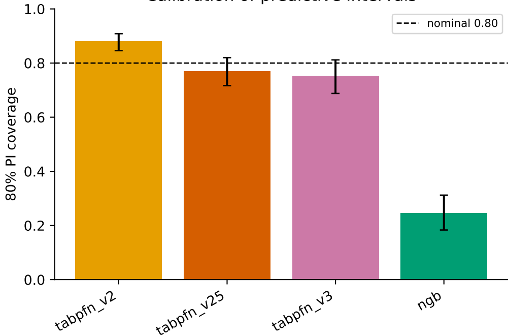
Calibration of predictive intervals
