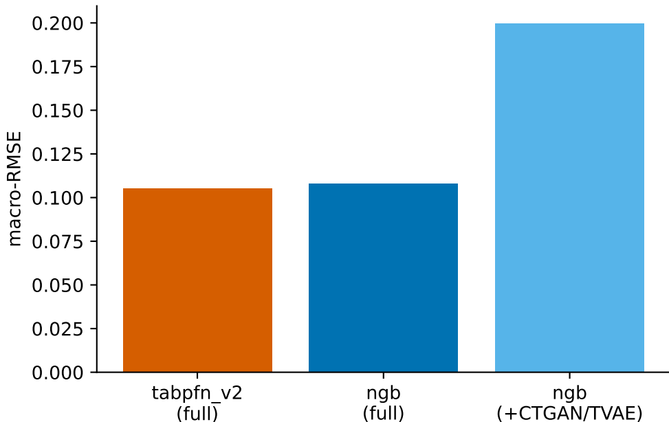
In-context TFM vs the augmentation pipeline (EBW)
