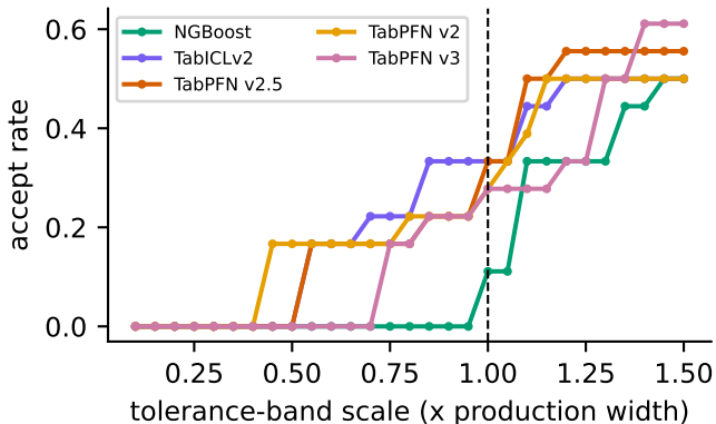
(a) accept rate vs band, \alpha=0.2
