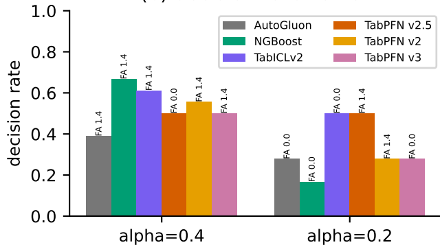
(b) decision rate vs risk
