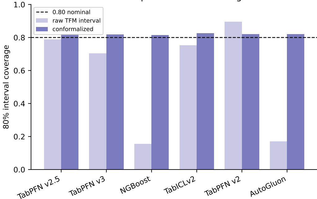
Raw vs split-conformal coverage
