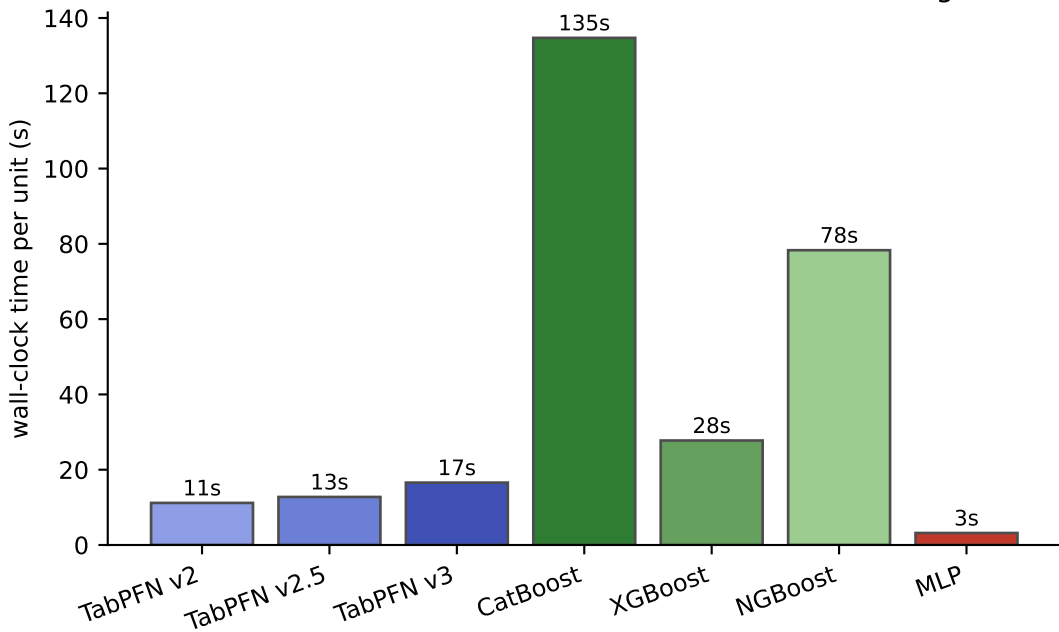
Cost: in-context inference versus nested-CV tuning
