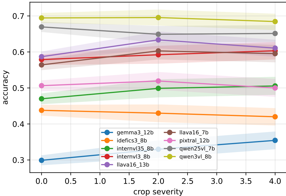
VizWiz robustness to crop
