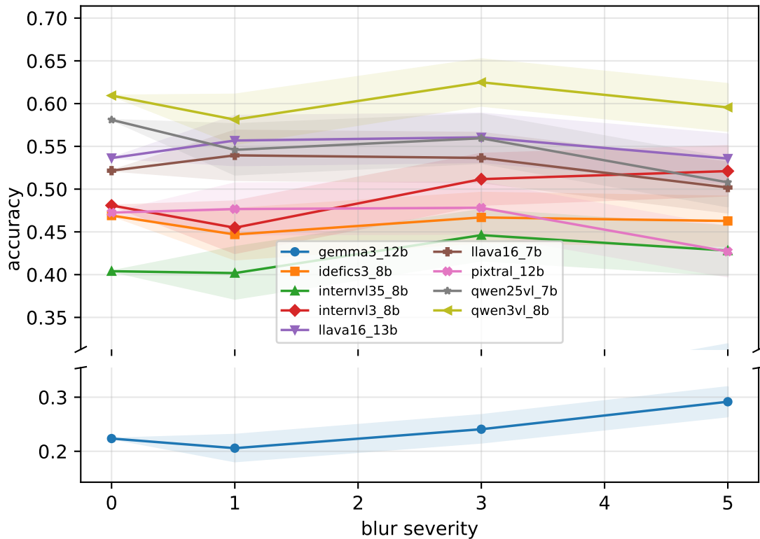
VizWiz ANSWERABLE robustness to blur
