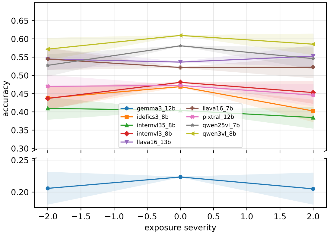
VizWiz ANSWERABLE robustness to exposure
