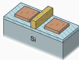
Lift-off
