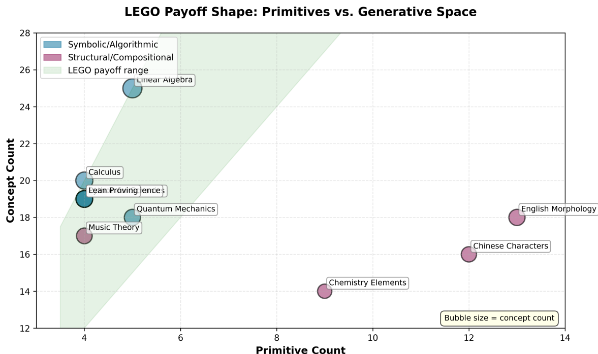
Figure 1: LEGO Payoff shape across ten representative domains. Each bubble represents a domain, with size proportional to the concept count. The x-axis shows primitive count (4–13), y-axis shows concept count (14–28). The shaded region (3–5x payoff) shows the typical generative space unlocked by a small primitive set. Symbolic/algorithmic domains cluster in blue; structural/compositional domains in purple. All domains exhibit the same compressive payoff structure.
