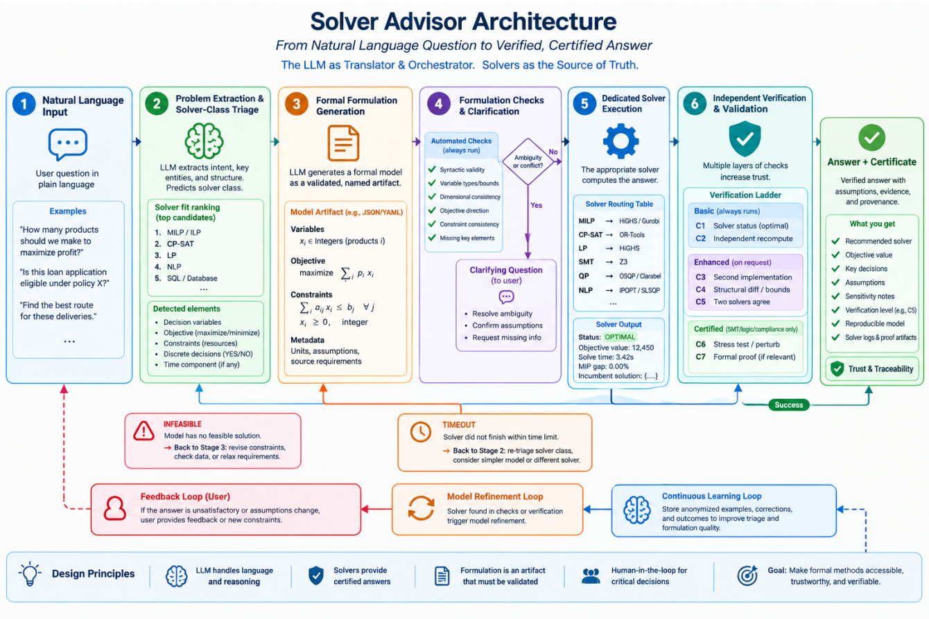
Figure 1: Solver Advisor Architecture
