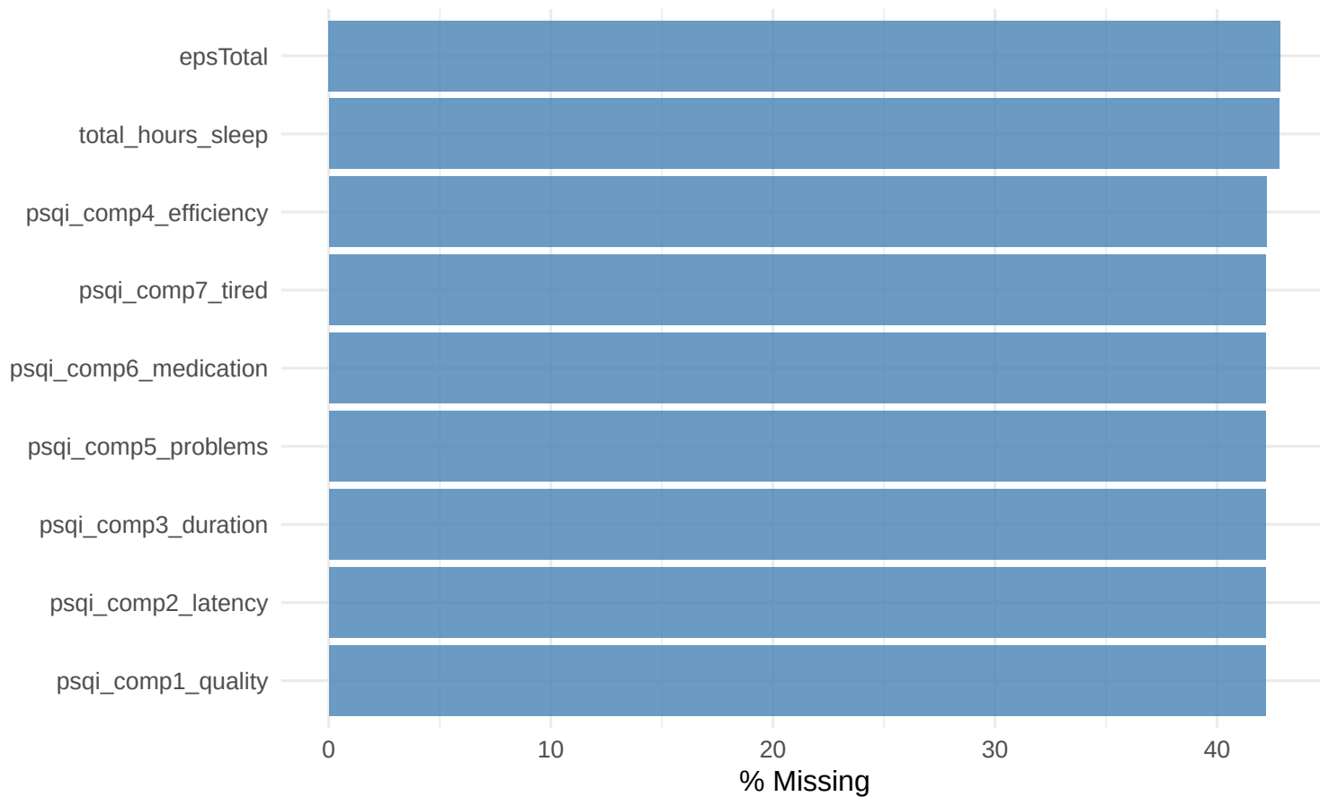
Proportion of Missing Data by Variable (panel_monthly)
