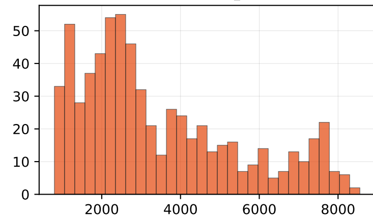
precipitation_sum
