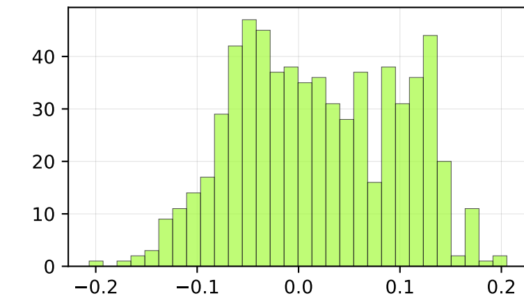
mean_temperature
