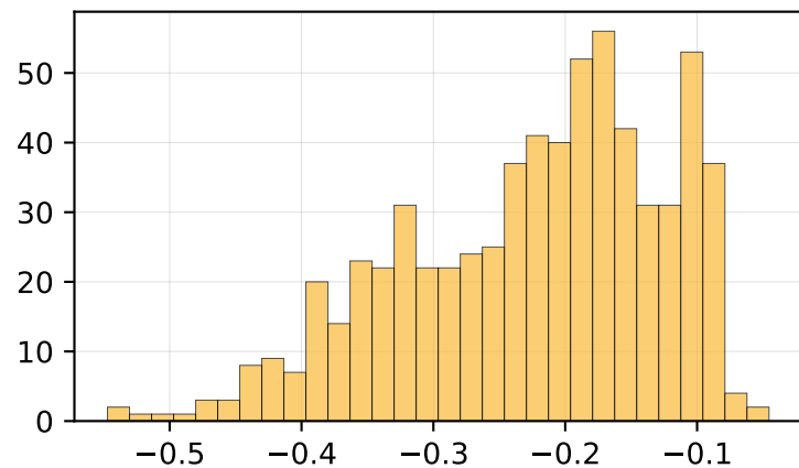
wetness
