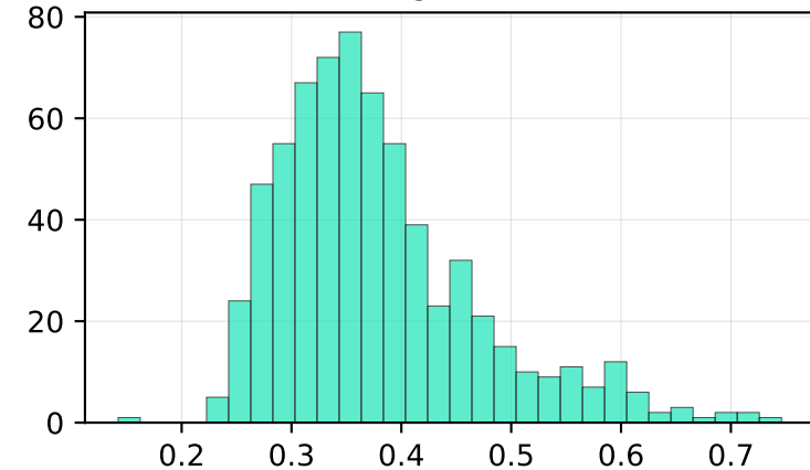
precipitation_sum
