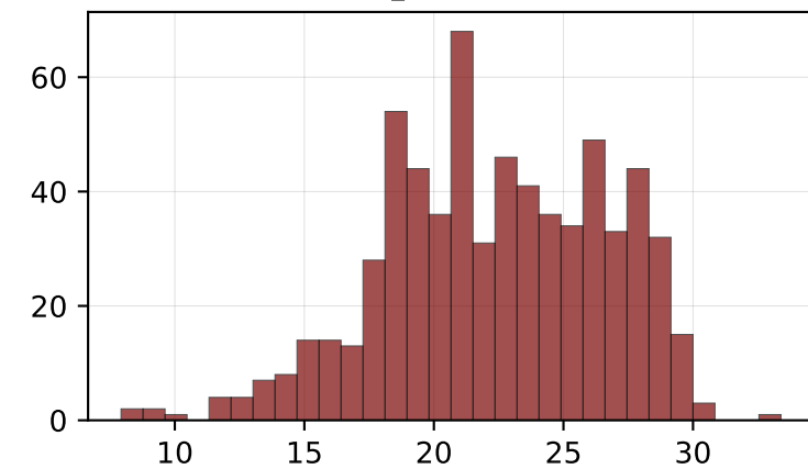
mean_temperature
