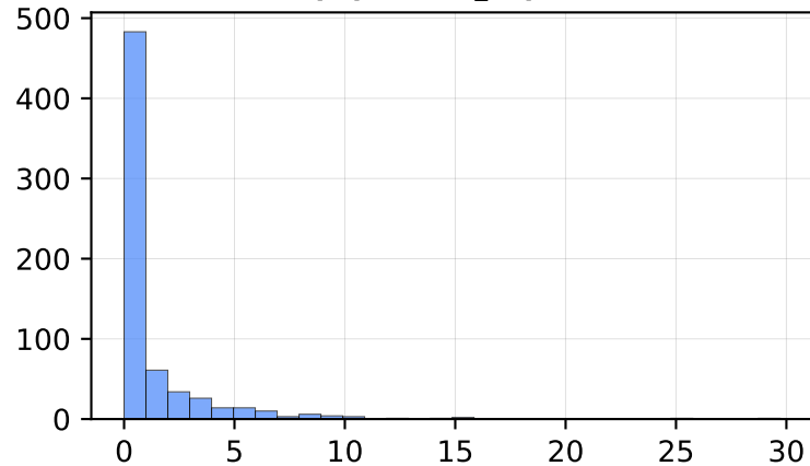
wetness
