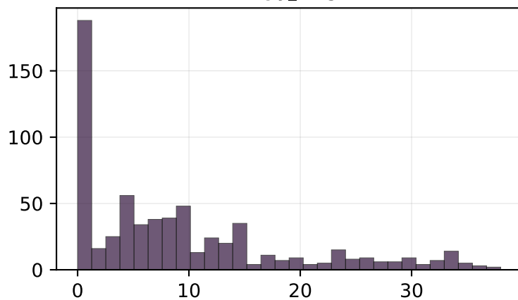
greenness
