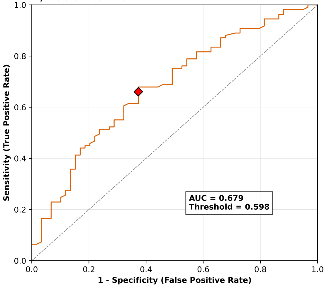
D) ROC Curve - TCI
