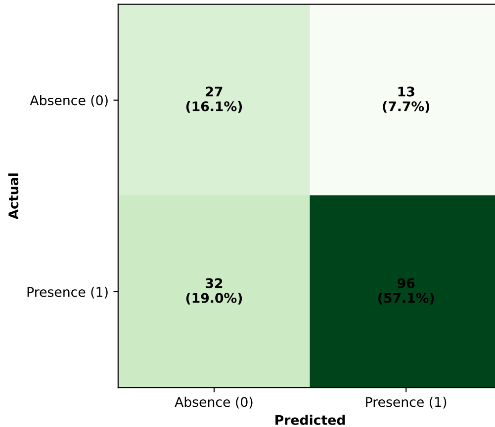
H) Confusion Matrix - GeoMAD
