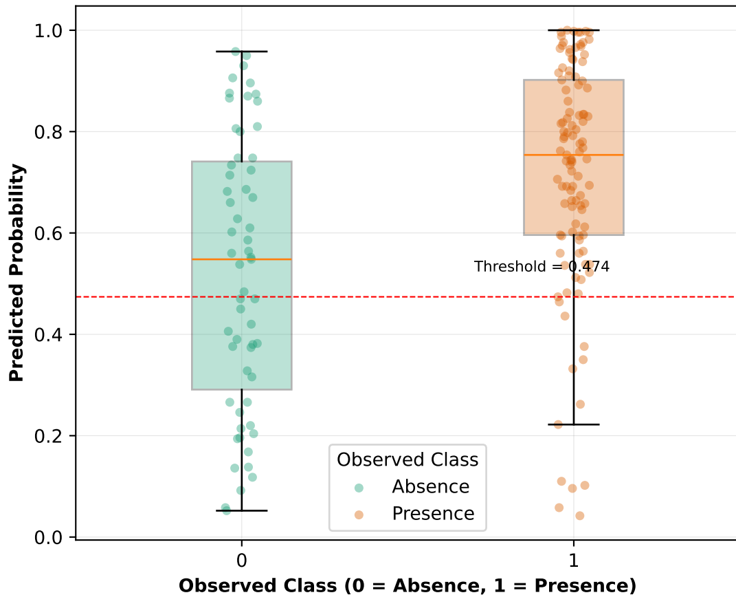
G) Model Predictions - GeoMAD
