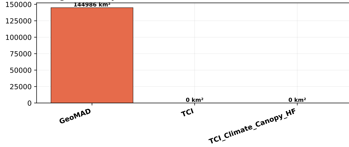
B) High Diversity Area Estimates
