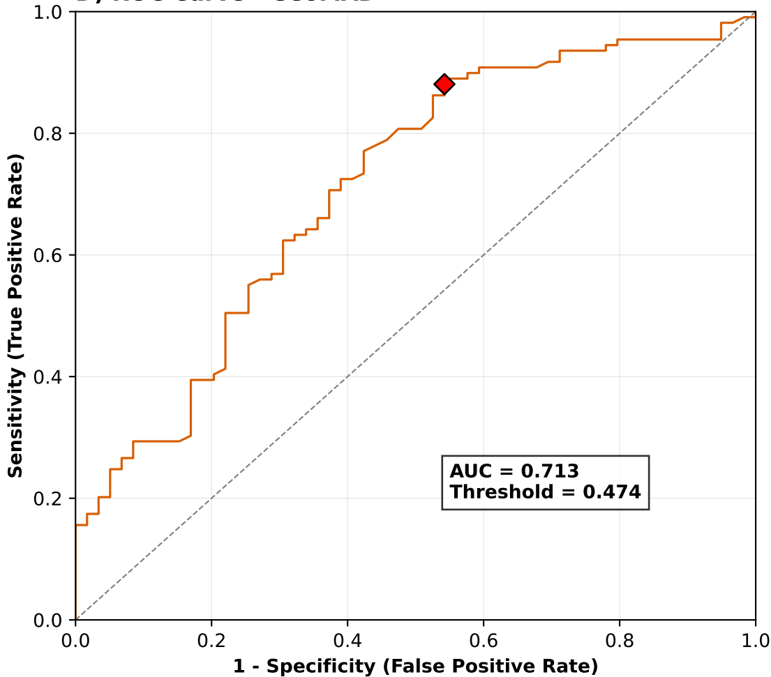
D) ROC Curve - GeoMAD
